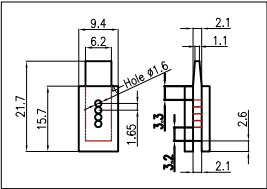
⑦ SPKR Unit BUSING
